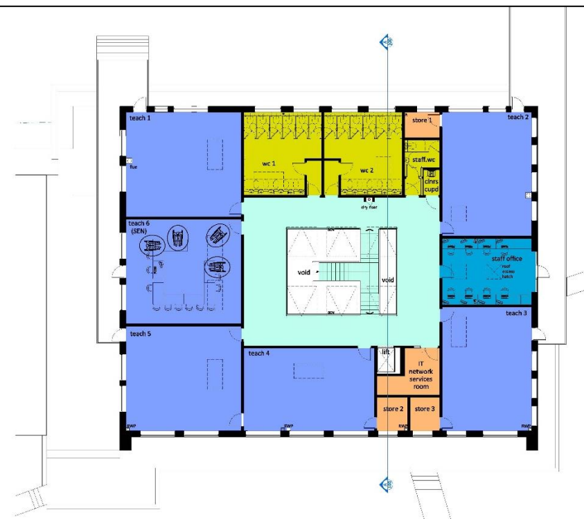
01 FIRST FLOOR 1:100 @ A1 1:300 @ A3
